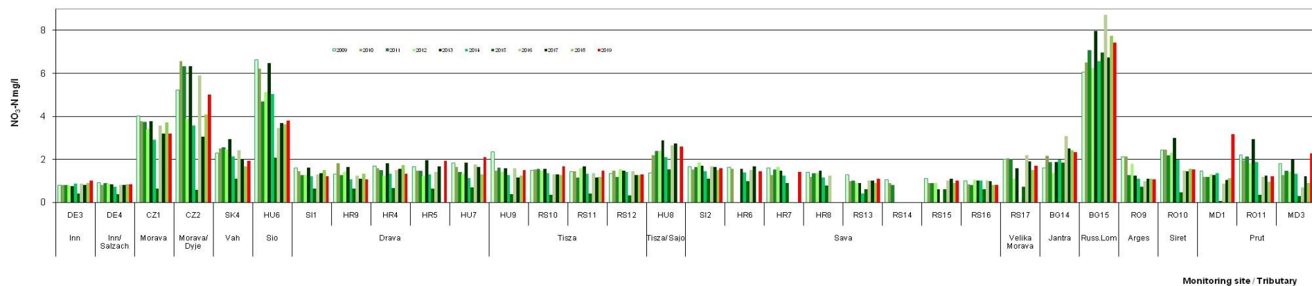
Figure 4.10.: Temporal changes (2009-2019) of NO 3 -N (c90) in tributaries.
