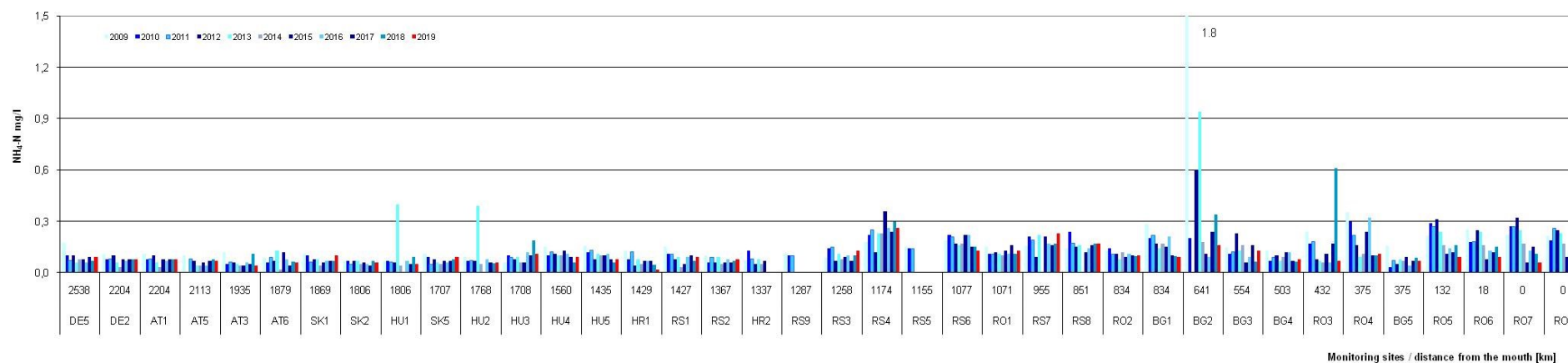
Figure 4.8.: Temporal changes (2009-2019) of NH 4 -N (c90) in tributaries.
