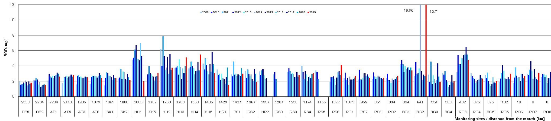
Figure 4.4.: Temporal changes (2009-2019) of BOD 5 (c90) in tributaries.
