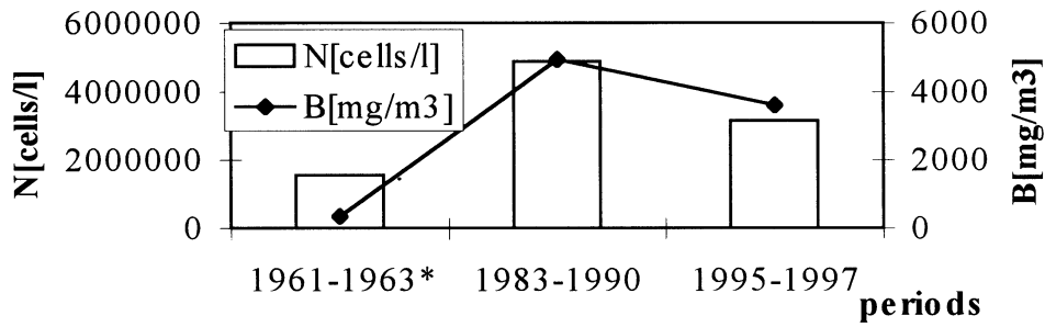
Figure 6 Phytoplankton abundance and biomass during different time-intervals (after Petrova, 1965)
