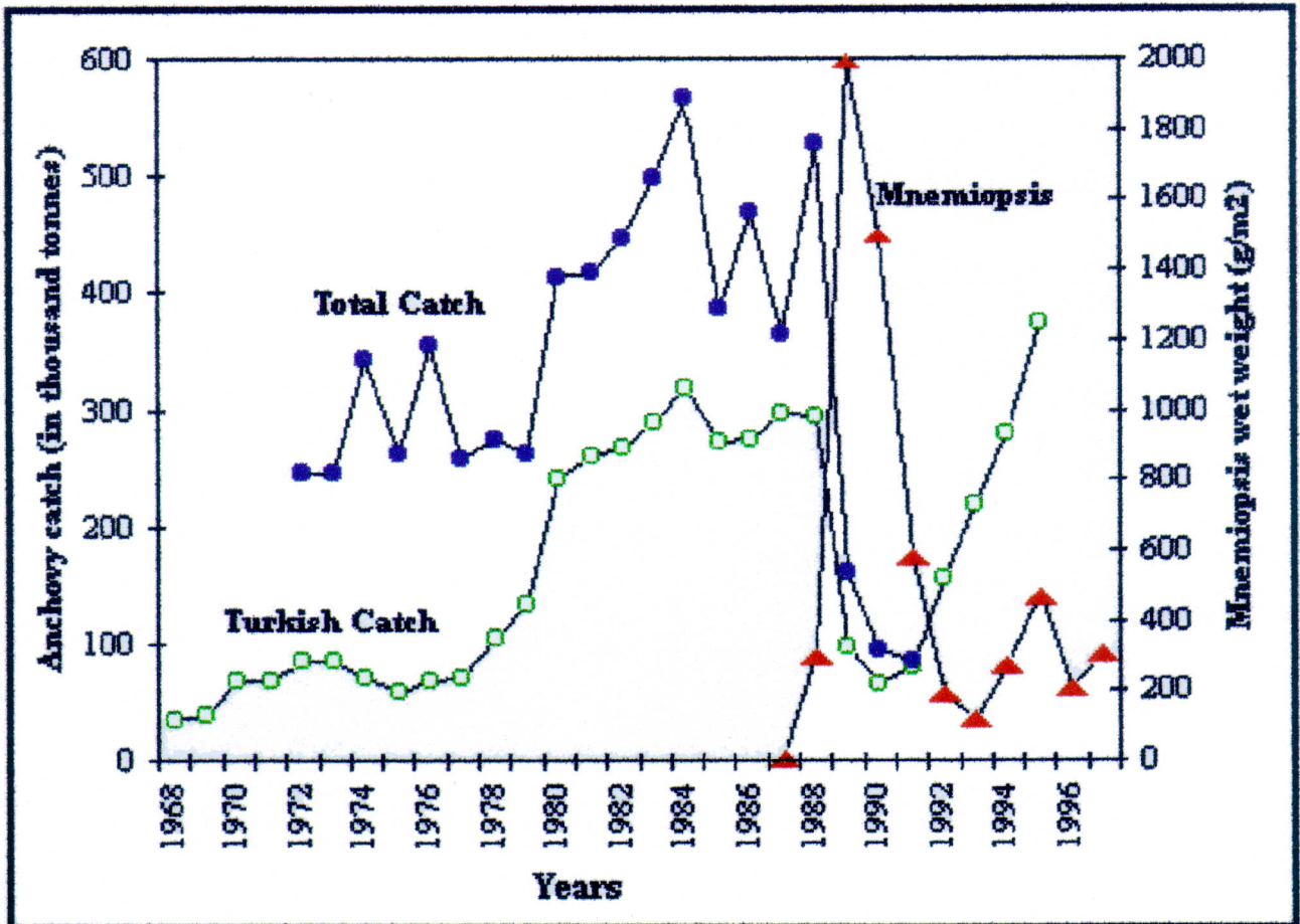
Figure 14 Anchovy catch values for the Black Sea. Open circles = Turkish catch, dark circles = total catch of all riparian countries, the dark triangles = biomass of Mnemiopsis leydii . No total catch available since 1991. The Mnemiopsis sp. biomass is expressed in area-specific terms. The data are by Kideys et al., 1998.
