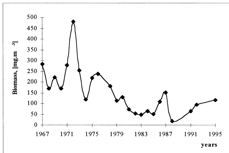
Figure 10 Long-term dynamic (1967-1995) of summer zooplankton biomass (without Noctiluca scintillans , Mnemiopsis leidyi and Scyphozoa) off the Bulgarian Coast (Konsulov A. and L. Kamburska, 1997)
