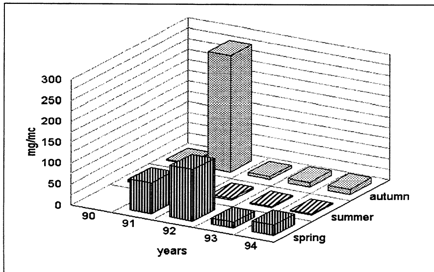
Figure 9 Seasonal evolution of the fodder zooplankton (1983-1994) in the shallow waters of the Romanian shelf
