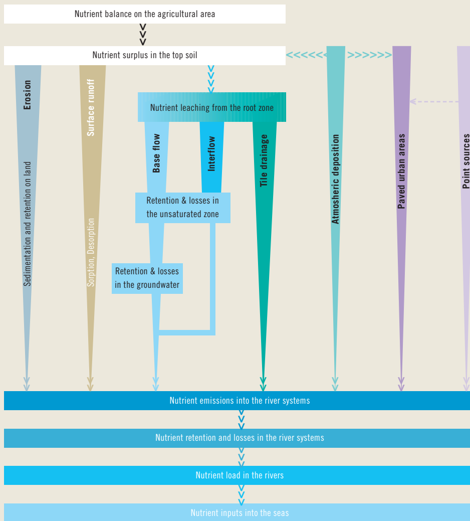
Pathways and processes used in MONERIS
