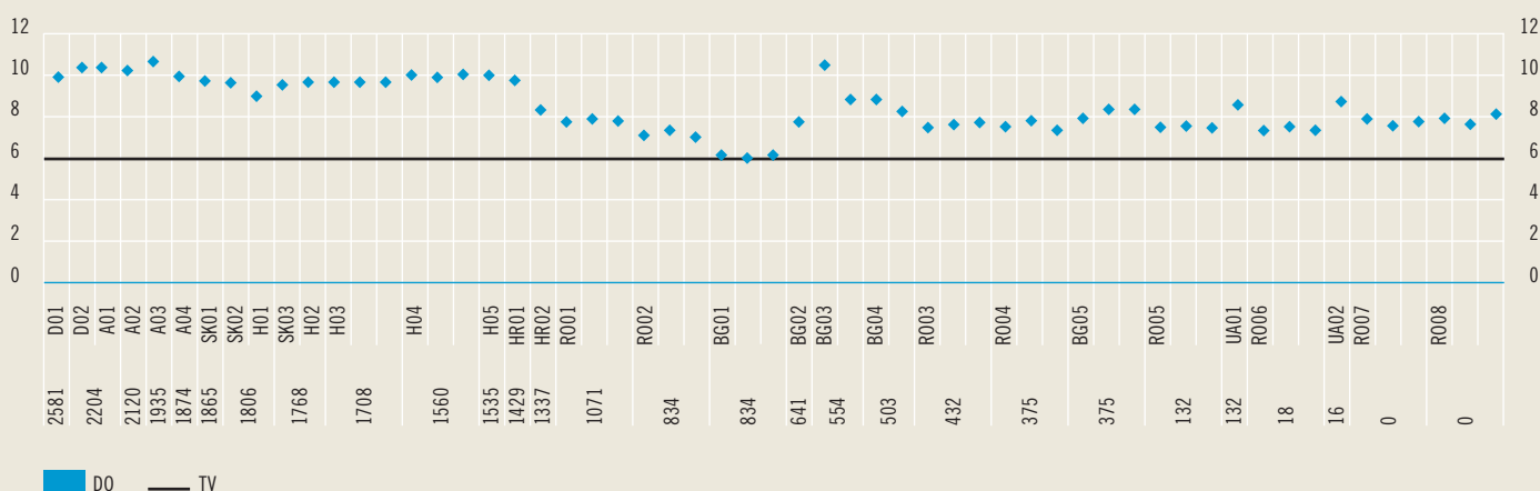
Dissolved Oxygen (DO) – Spatial distribution of mean values of c10 for 1996 - 2000 data against the limit of Class II (TV - target value) – the Danube River. Contrary to the other determinands, in the case of dissolved oxygen the “above target value” means a favorable situation
